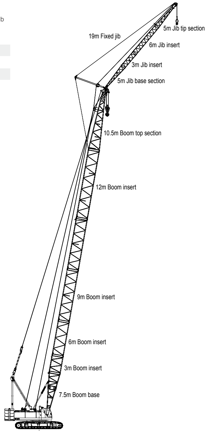
57m boom + 19m Jib
